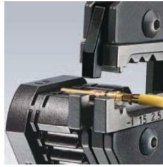
97 43 200 with crimping dies 97 49 61 and revolvable locator 97 49 90 for tuned types of connectors with varying pin diameters
